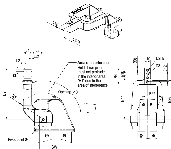
Vertical clamping arm position
