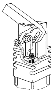
Roller and cam mechanism of the models 870-2 and 871-2
