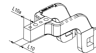
U-clamp arms, central
