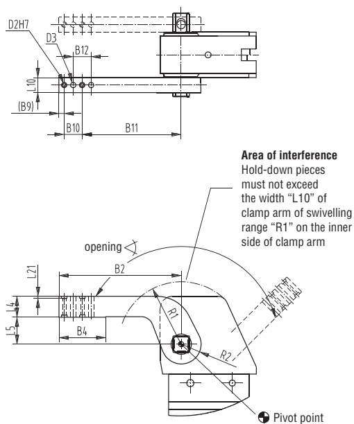
Horizontal clamping arm position
